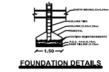
FOUNDATION DETAILS
