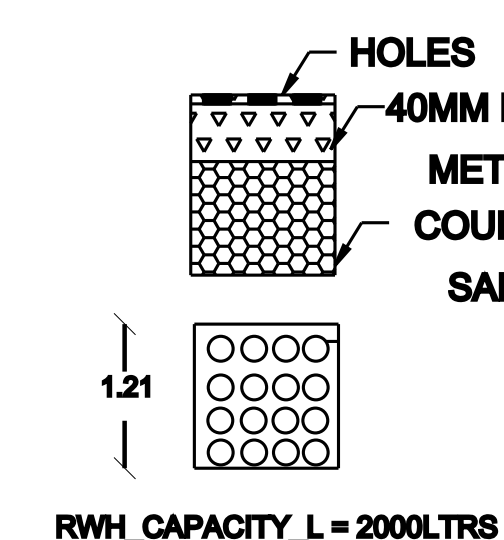
RAIN WATER COLLECTING TANK
