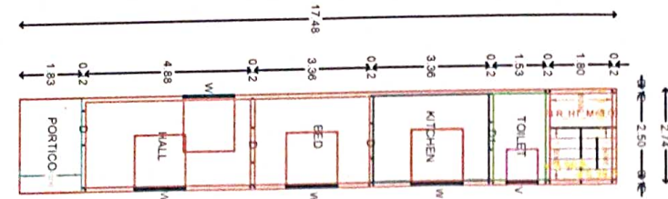
G.FLOOR PLAN
