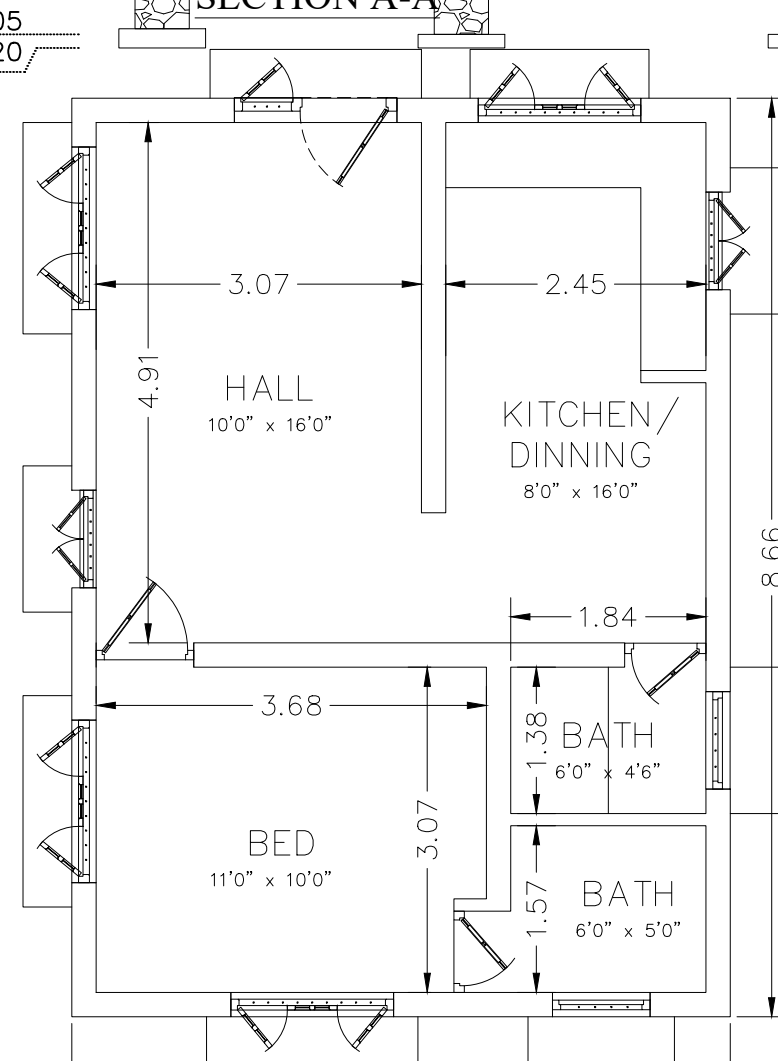
EX., GROUND FLOOR PLAN
