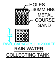
RAIN WATER COLLECTING TANK
