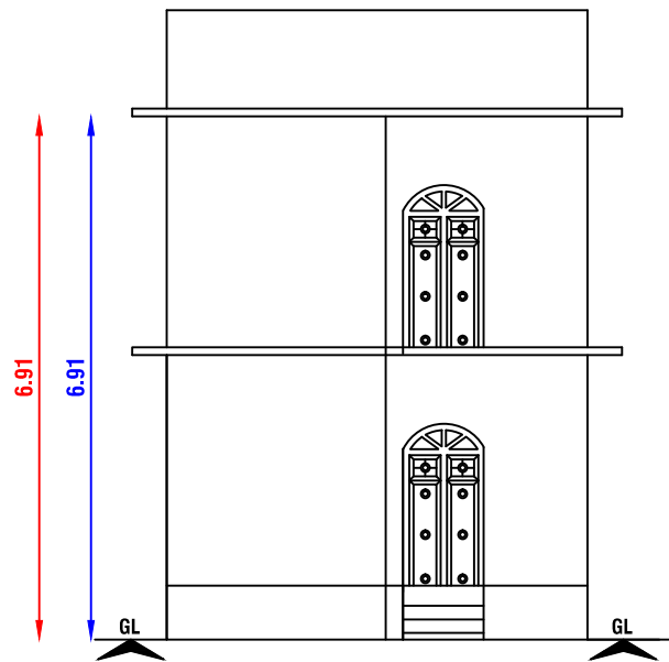
FRONT ELEVATION
