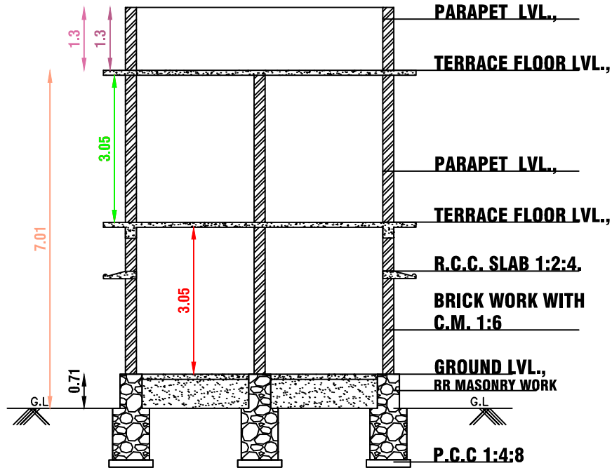
SECTION ON A-A & A'-A'
