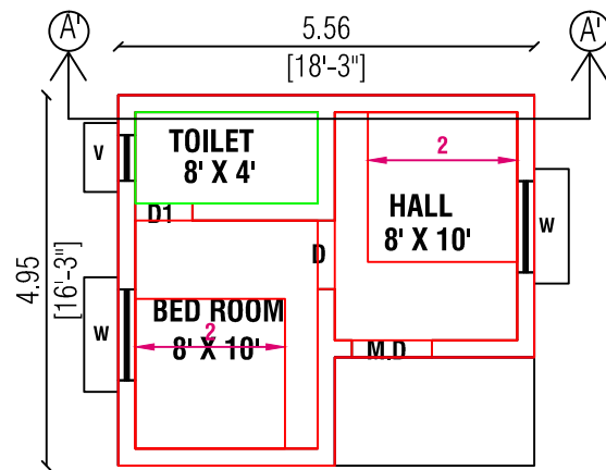
PRO.FIRST FLOOR PLAN
