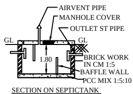
SECTION ON SEPTICTANK
