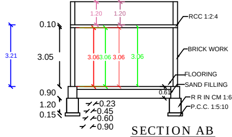
SECTION AB
