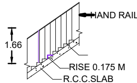
STAIRCASE
