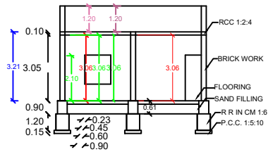
SECTION AB
