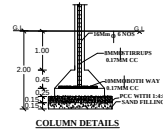
COLUMN DETAILS
