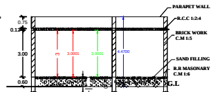
SECTION ON "BB"
