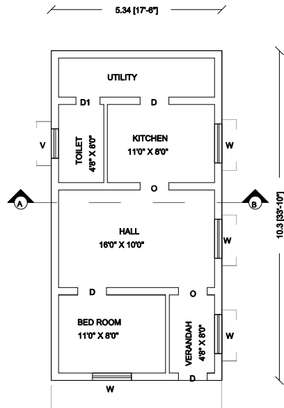
PLAN
