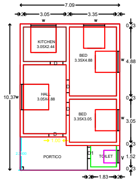
G.FLOOR PLAN
