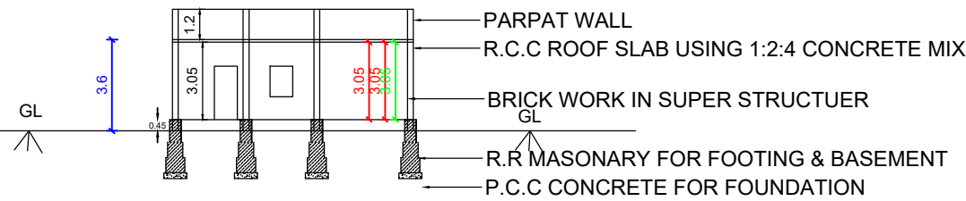
SECTION ON AB
