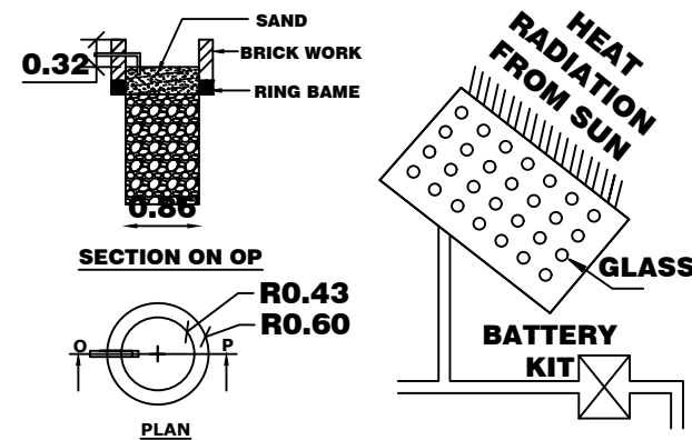
SOLAR SYSTEM
