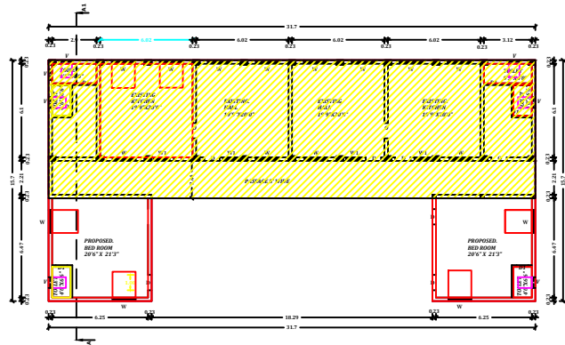
PROPOSED / EXISTING. GROUND FLOOR PLAN
