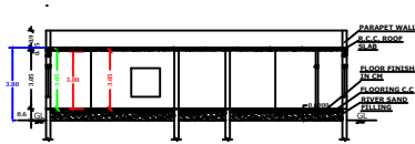
SECTION ON AA1
