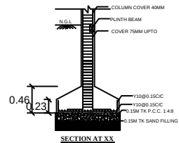
SECTION AT XX
