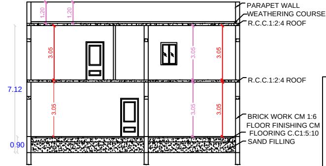
SECTIONON SV
