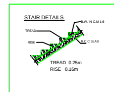
STAIR DETAILS
