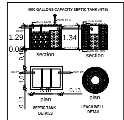
1000 GALLONS CAPACITY SEPTIC TANK (NTS)
