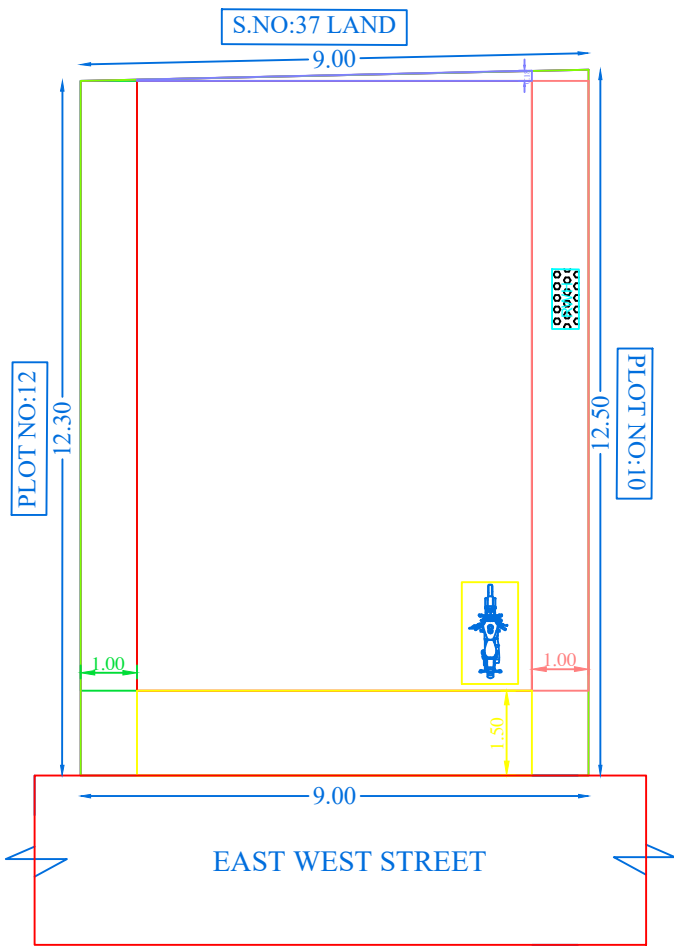
SITE PLAN
