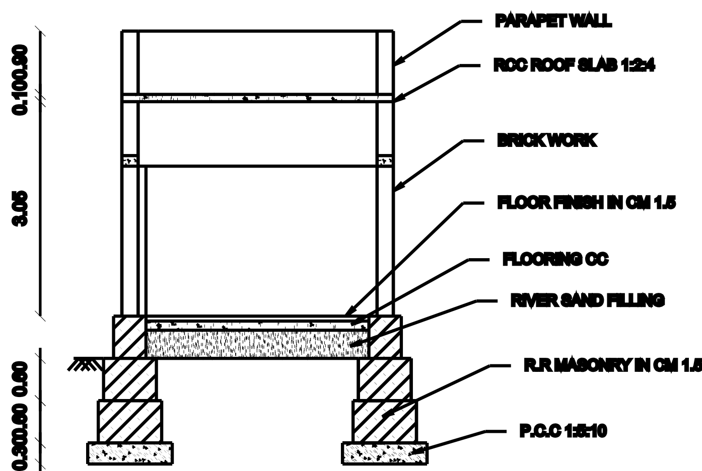
SECTION AA1
