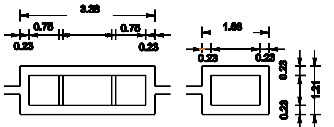
PLAN & SECTION OF SEPTIC TANKU TRAP PROVIDED
