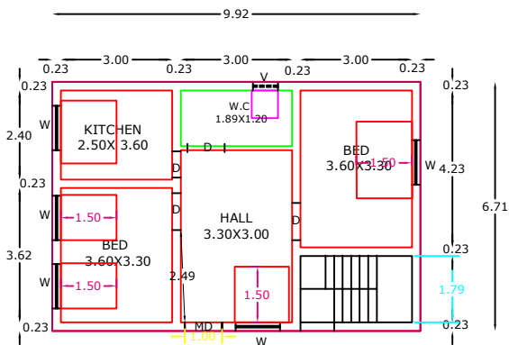
PRO GROUND FLOOR RESIDENTIAL PLAN
