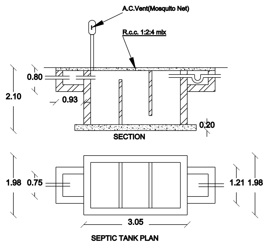
SEPTIC TANK PLAN
