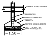
FOUNDATION DETAILS
