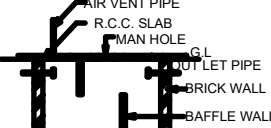
SECTION ON SEP.TANK
