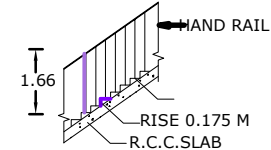
STAIRCASE
