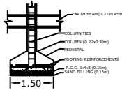
FOUNDATION DETAILS
