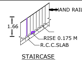
STAIRCASE
