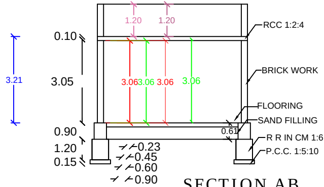
SECTION AB
