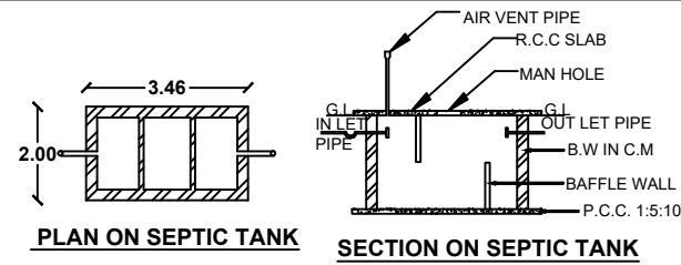
SECTION ON SEPTIC TANK
