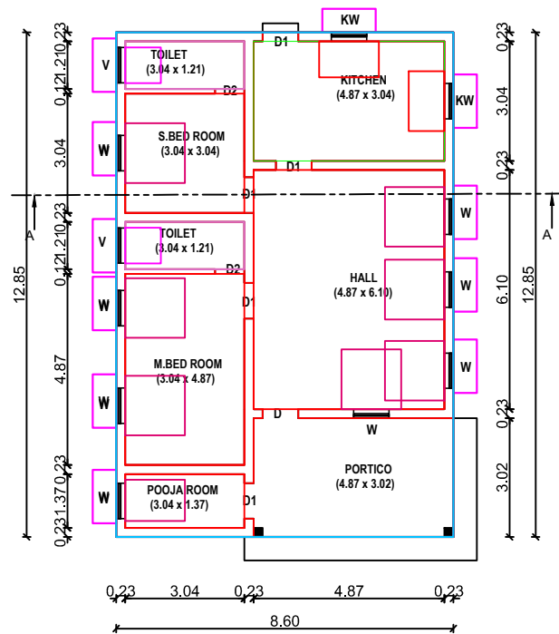
PLAN
