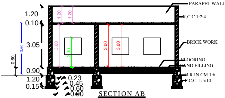
SECTION AB
