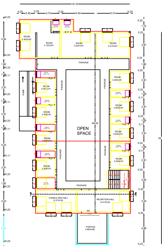
EXT GROUND FLOOR COMMERCIAL PLAN
