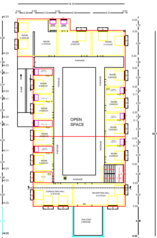
EXT FIRST FLOOR COMMERCIAL PLAN
