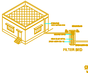
PRO.RAIN WATER SYSTEM
