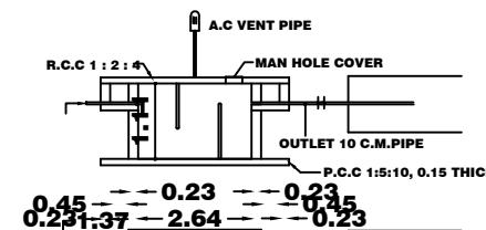
SEPTIC TANK & TRENCH
