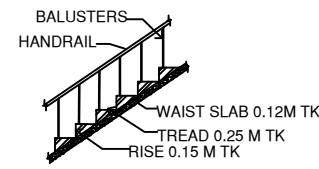
STAIRCASE DETAILS
