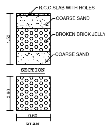
RAIN WATER HARVESTING
