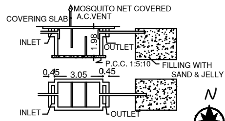
SEPTIC TANK & TRENCH U TRAP PROVISION
