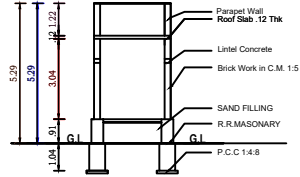
SECTION ON AB
