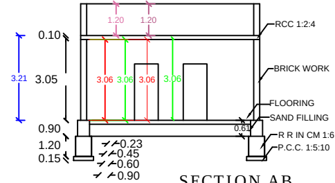
SECTION AB
