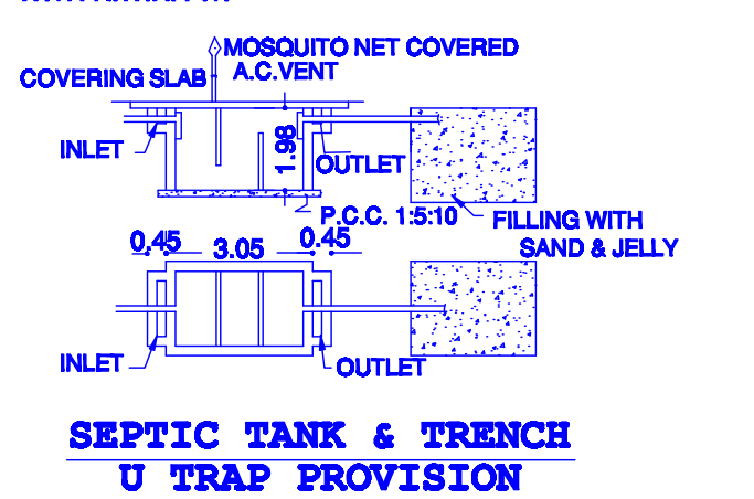
SEPTIC TANK & TRENCH U TRAP PROVISION
