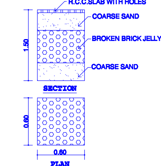
RAIN WATER HARVESTING
