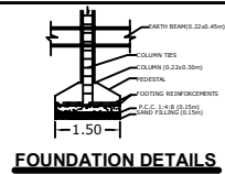
FOUNDATION DETAILS
