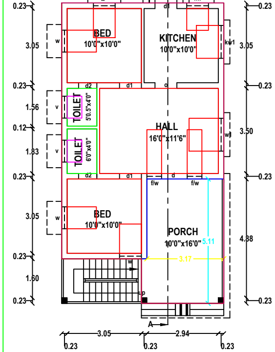
PLAN - GROUND FLOOR RESIDENCE
