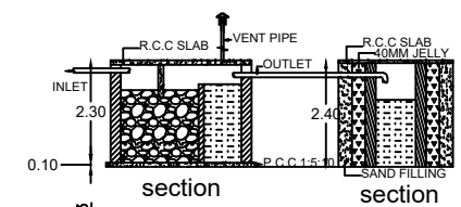
1000 GALLONS CAPACITY SEPTIC TANK (NTS)
