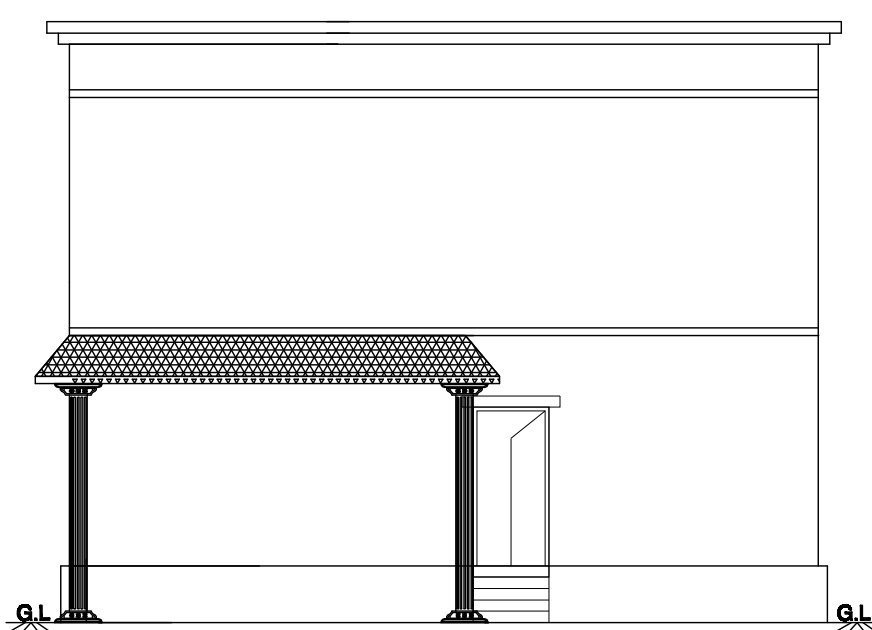
FRONT ELEVATION
