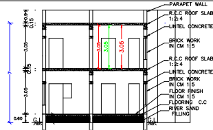
SECTION ON AA1
