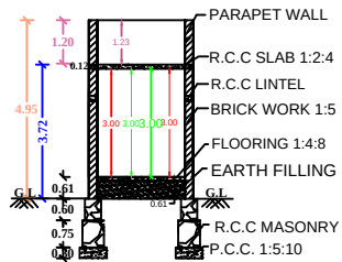
"SECTION "AB"
