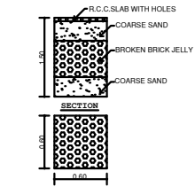
RAIN WATER HARVESTING
