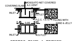
SEPTIC TANK & TRENCH U TRAP PROVISION
