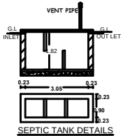
SEPTIC TANK DETAILS
