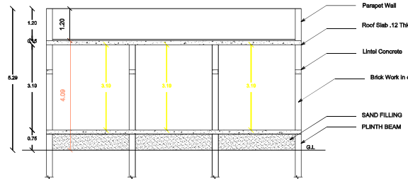
SECTION ON R-K
