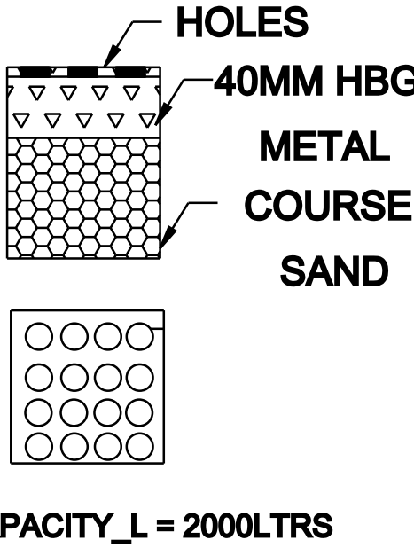
RAIN WATER COLLECTING TANK
