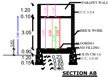
SECTION AB
