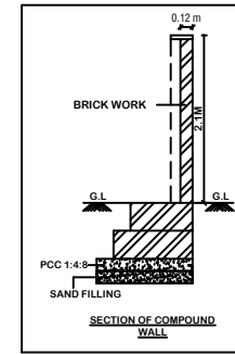
SECTION OF COMPOUND WALL
