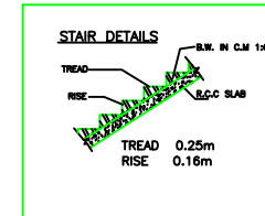
STAIR DETAILS
