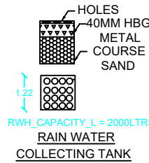
RAIN WATER COLLECTING TANK
