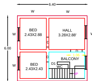
FIRST FLOOR RESIDENTIAL PLAN
