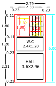
EXT GROUND FLOOR RESIDENTIAL PLAN
