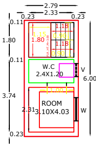
PRO FIRST FLOOR RESIDENTIAL PLAN
