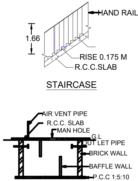
SECTION ON SEP.TANK
