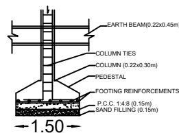
FOUNDATION DETAILS
