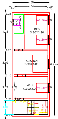
EXT GROUND FLOOR RESIDENTIAL PLAN
